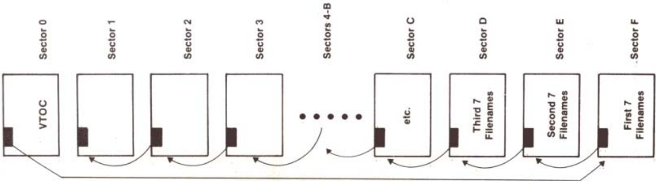
FIGURE 4.3 — TRACK 17, THE CATALOG TRACK
