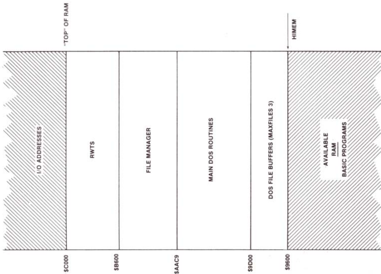
FIGURE 5.1 — DOS MEMORY USE (48K APPLE)
